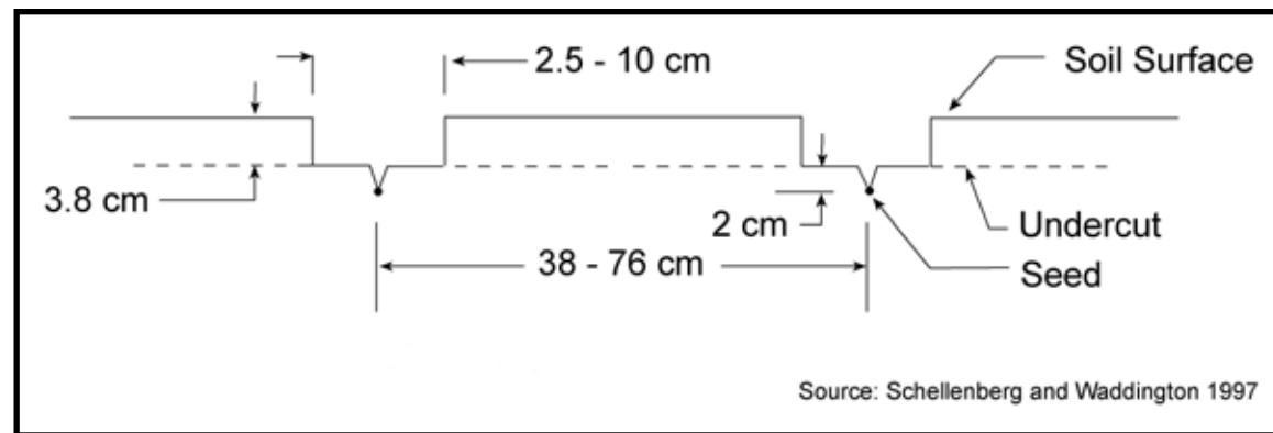
Legend: 3.8 cm = 1.5 in, 38-76 cm = 15-30 in, 2 cm = 0.5 in, 2.5-10 cm = 1-4 in Figure 17. Slotseeding technique used in the study.
