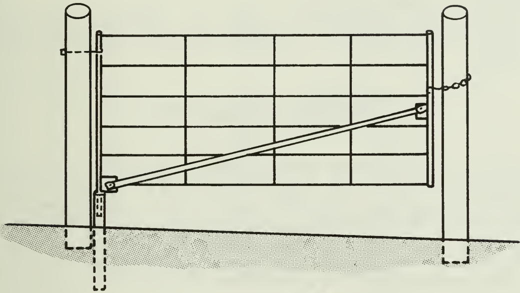
Fig. 44 Hanging gate at 45° allows it to swing fully back against fence.
