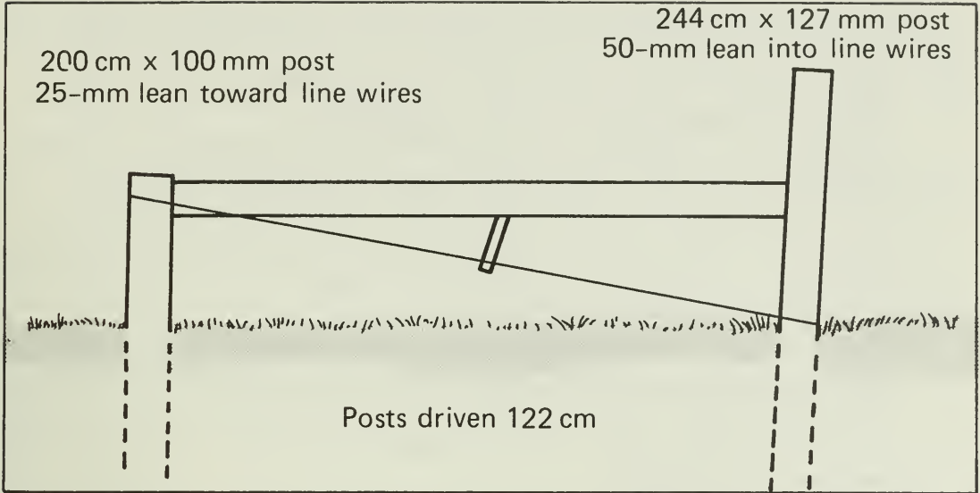
Fig. 31 Medium corner brace assembly (Fig. 30) showing construction.
